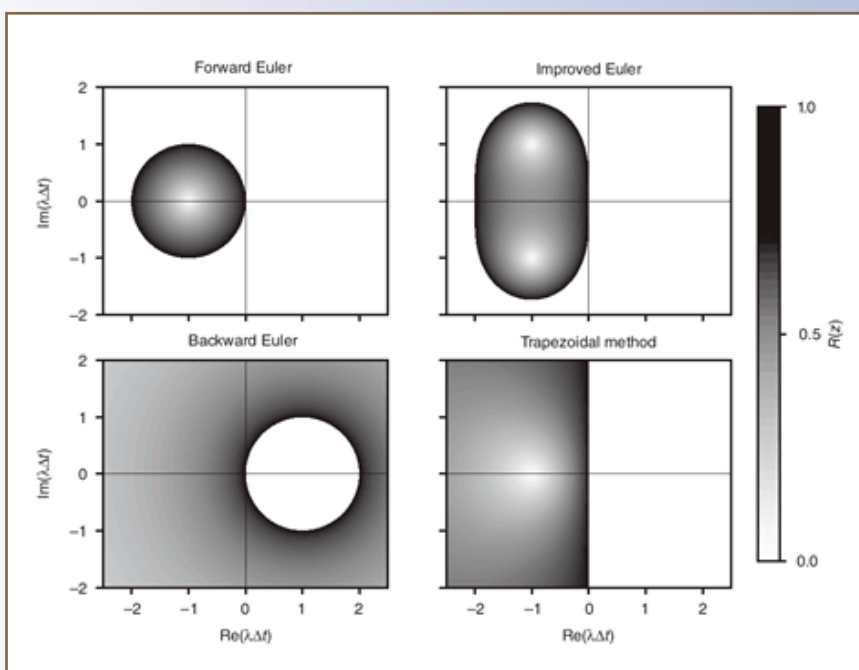
Figure 1: Stability region of different Euler time-integration methods This is Figure 7.7 in the book
