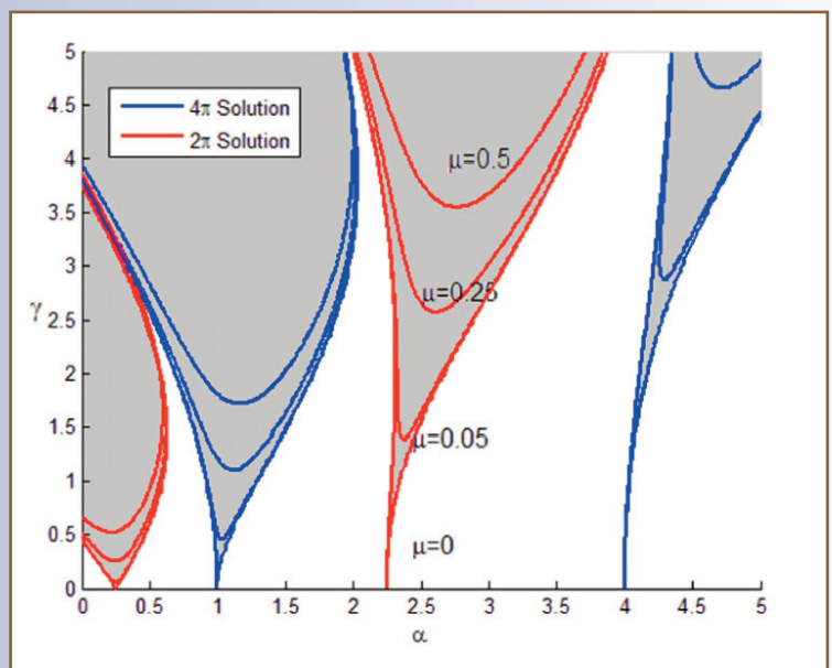
Figure 3: The Ince-Strutt diagram showing regions of stability and instability for the Mathieu equation. A black-white version of this diagram appears as Figure 9.2 in the book. The color version shown here is taken from the paper by H. Moideen, J.M. Falzarano and S.A. Sharma, Ocean Systems Eng., Vol. 2, pp. 239-255, 2012, published by Techno-Press Journals
