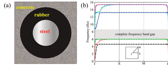
Figure 2: (a) Unit cell configuration. (b) In-plane elastic modes of a square lattice of steel cylinder coated with rubber polymer in a concrete matrix. The inset shows the first irreducible Brillouin zone [6]
