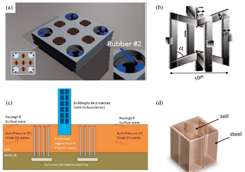
Figure 3: (a) Composite layered structures with attenuation zone [10]; (b) negative Poisson's ratio seismic metamaterials [11]; (c) seismic metamaterials clamped to bedrock [12]; and (d) low frequency and large-scale phononic crystals [13]
