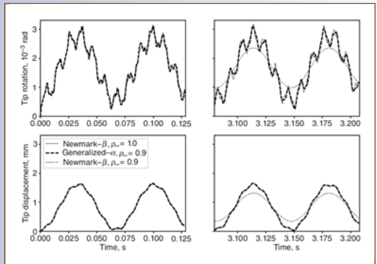
Figure 2: Comparison of Newmark and Generalized- \alpha (HHT) methods This is Figure 7.21 in the book
