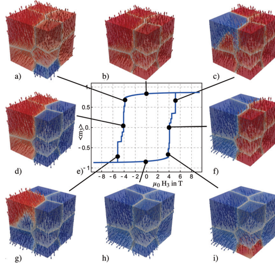
Figure 4: a)-d) & f)-i) polycrystalline hard magnetic microstructure under alternating external magnetic field H_3 and magnetization vectors \mathbf{m} , and e) effective hysteresis loop [15]
