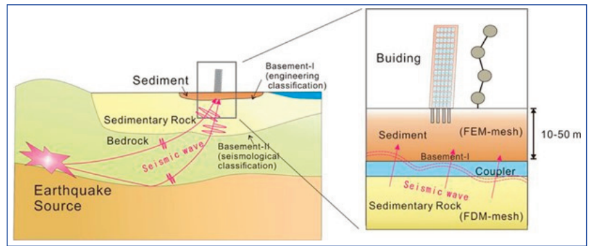
Figure 1: Propagation mechanism of seismic wave [4]
