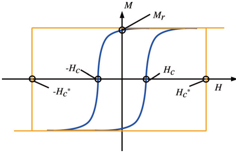
Figure 3: Illustration of theoretical (yellow) and experimentally (blue) observed hysteresis curves
